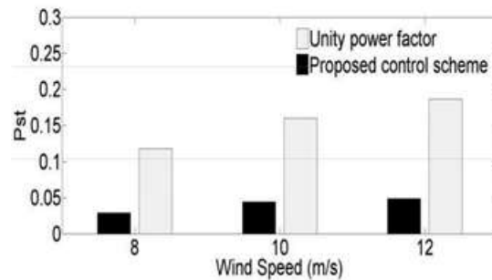
Fig. 8. Pst values vs. average wind speed at a turbulence intensity of 15 %, X/R ratio of 2 and SC R of 3.
