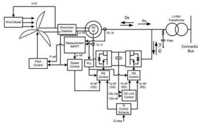
Fig. 2. DFIG control schematic.
