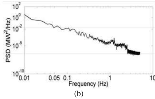
Fig. 3. Output power of the DFIG unit at an average wind speed of 10 m/s and turbulence intensity of 15 %: (a) ten-minute temporal plot, (b) corresponding power spectral density plot.
