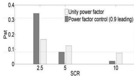
Fig. 4. Pst values vs. SCR under operation at a leading power factor at an X/R of 2, average wind speed of 10 m/s and turbulence intensity of 15 %.
