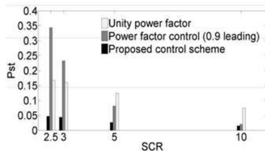
Fig. 9. Pst values vs. SC R under the proposed control scheme at an X/R ratio of 2, average wind speed of 10 m/s and turbulence intensity of 15 %.
