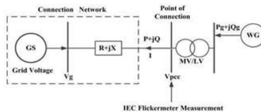
Fig. 1. Power system representation for WG flicker studies.
