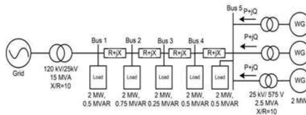
Fig. 11. Distribution feeder layout.
