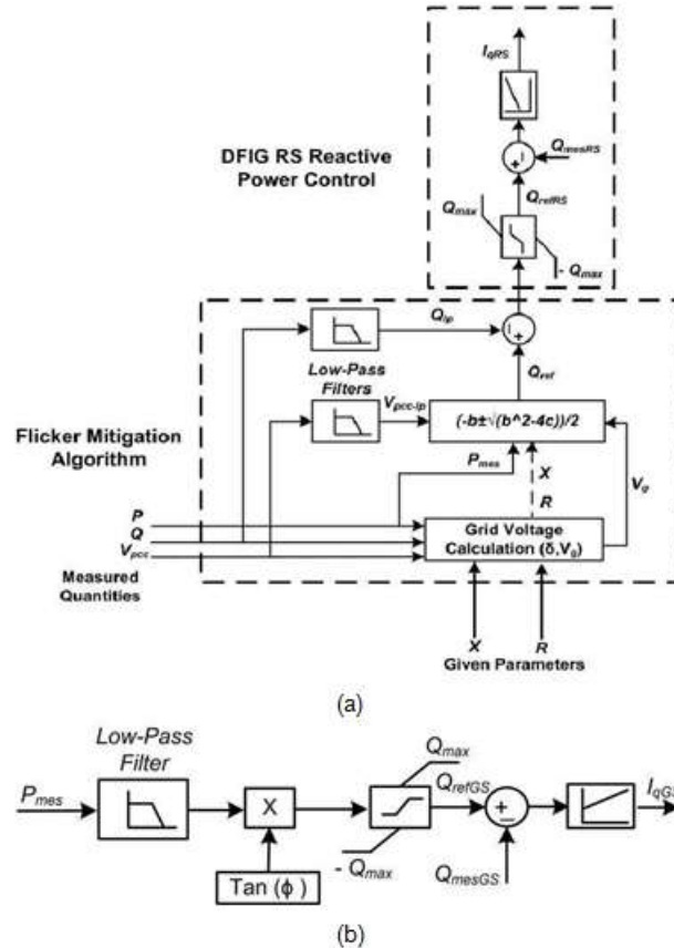
Fig. 6. Flicker mitigation control scheme: (a) RS reactive power control, (b) GS reactive power control. the proposed control scheme effectiveness for different site conditions (zero reactive power reference for the GS converter and network model as per [21]).
